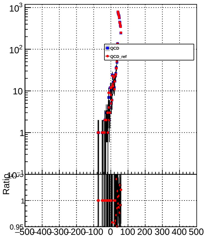
METResolution_GenMETTrue_MET40to60
