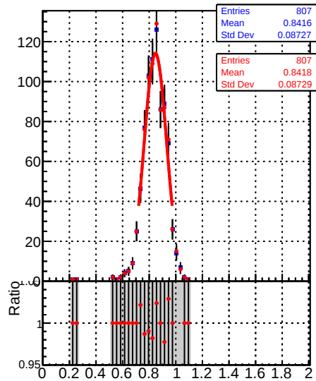
Raw Jet response ( pT/pT_{\text{gen}} ) in 153 \leq p_t < 196 , 2.1 \leq |\eta| < 2.5
