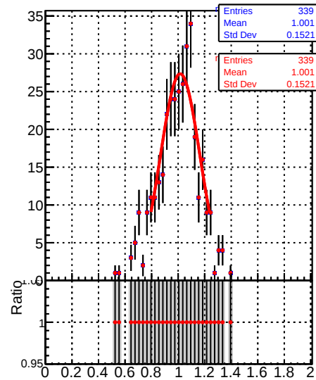
Raw Jet response ( pT/pT_{\text{gen}} ) in 153 \leq p_t < 196 , 3.0 \leq |\eta| < 5.0
