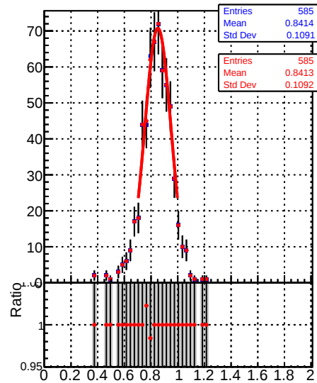
Raw Jet response ( pT/pT_{\text{gen}} ) in 153 \leq p_t < 196 , 2.5 \leq |\eta| < 3.0
