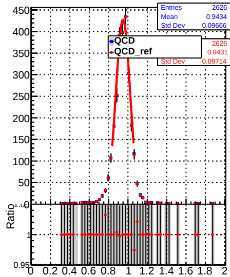
Raw Jet response ( pT/pT_{\text{gen}} ) in 153 \leq p_t < 196 , 0.0 \leq |\eta| < 0.5
