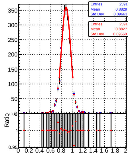
Raw Jet response ( pT/pT_{\text{gen}} ) in 153 \leq p_t < 196 , 1.3 \leq |\eta| < 2.1
