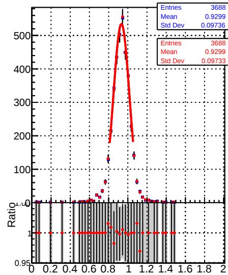
Raw Jet response ( pT/pT_{\text{gen}} ) in 153 \leq p_t < 196 , 0.5 \leq |\eta| < 1.3
