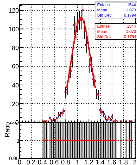
Jet response (pT/pTgen) in 49 <= pt < 64, 3.0 <= |eta| < 5.0
