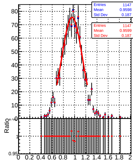
Jet response (pT/pTgen) in 49 <= pt < 64, 2.5 <= |eta| < 3.0
