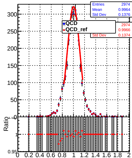
Jet response (pT/pTgen) in 49 <= pt < 64, 0.0 <= |eta| < 0.5
