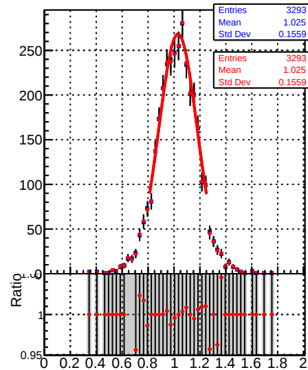
Jet response (pT/pTgen) in 49 <= pt < 64, 1.3 <= |eta| < 2.1
