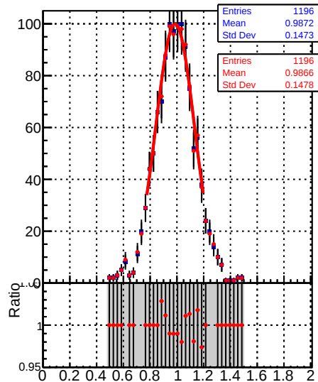
Jet response (pT/pTgen) in 49 <= pt < 64, 2.1 <= |eta| < 2.5
