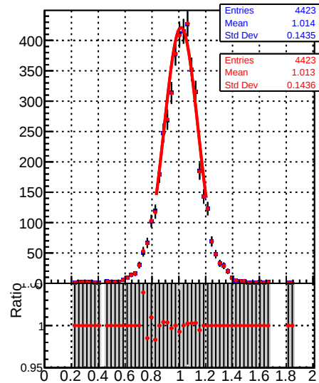
Jet response (pT/pTgen) in 49 <= pt < 64, 0.5 <= |eta| < 1.3
