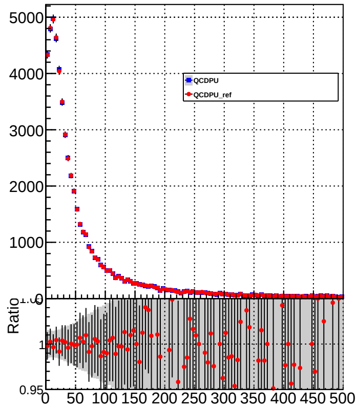
neutralHadronEnergy
