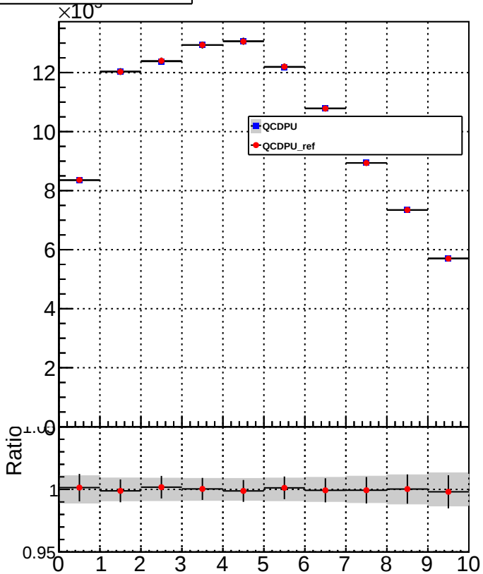
photonMultiplicity
