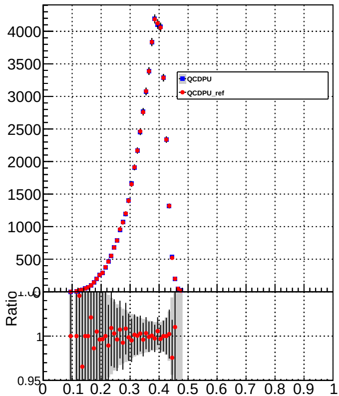
HFHadronEtFraction
