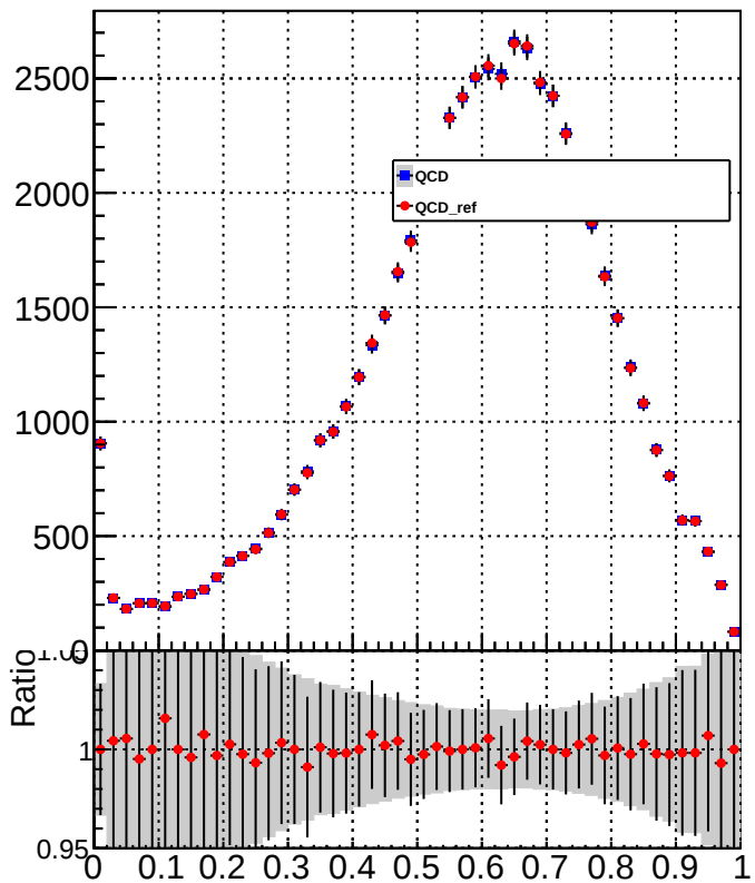
chargedHadronEnergyFraction
