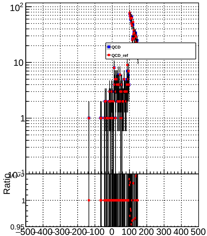
METResolution_GenMETTrue_MET100to150
