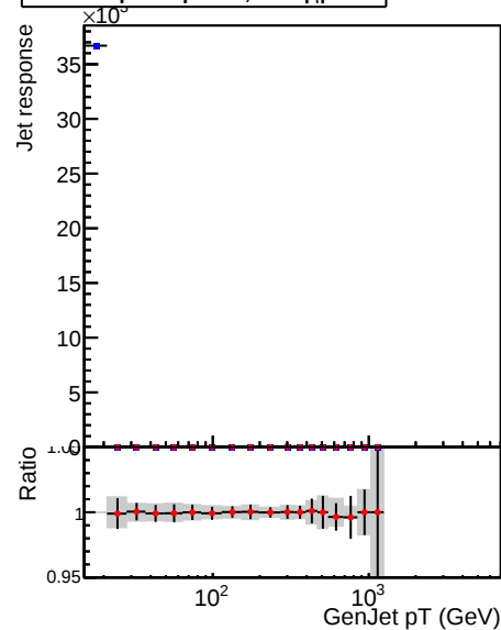
Raw Jet pT response, 2.1 < |\eta| < 2.5
