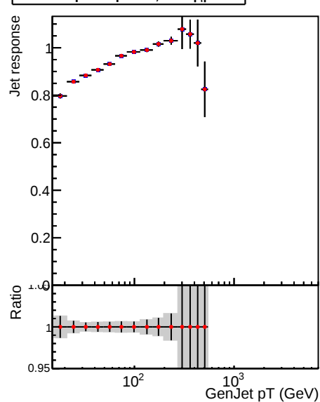
Raw Jet pT response, 3.0 < |\eta| < 5.0
