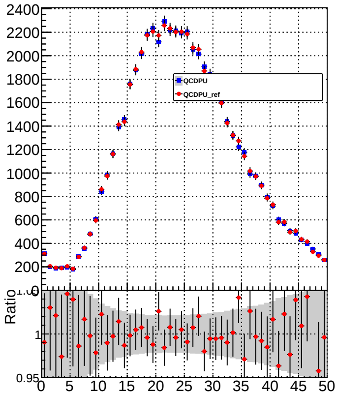
chargedHadronMultiplicity
