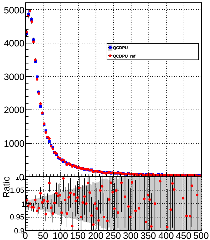
neutralHadronEnergy
