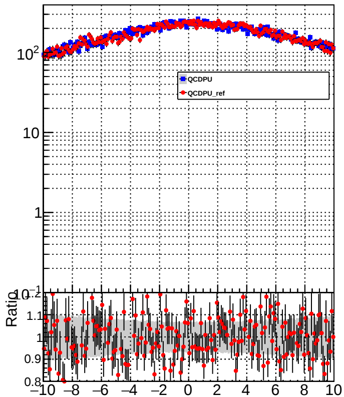
METUnc_JetResDown
