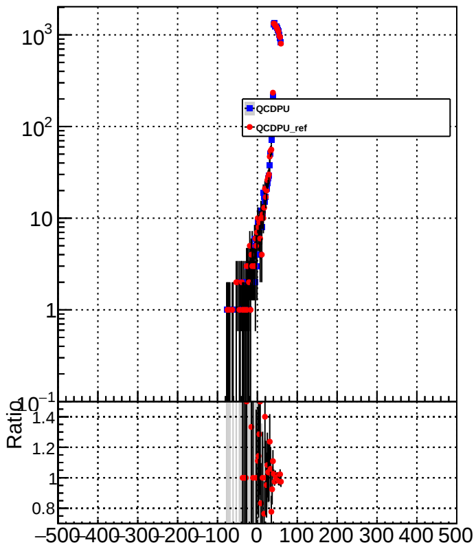
METResolution_GenMETTrue_MET40to60
