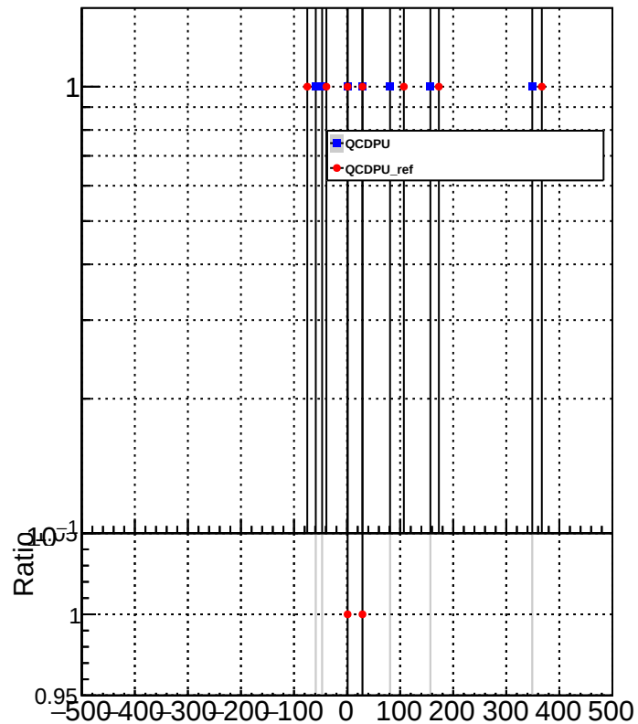
METResolution_GenMETTrue_MET500
