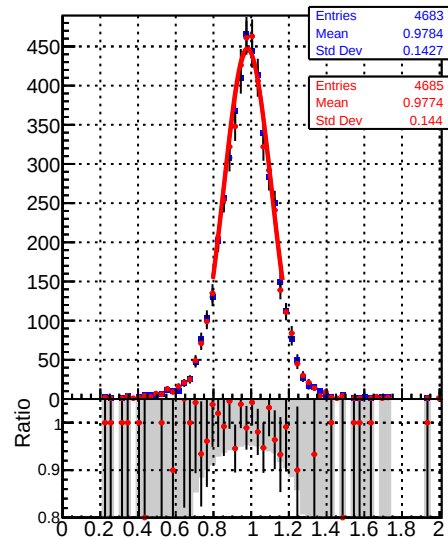
Jet response ( p_T/p_{T\text{gen}} ) in 84 \leq p_t < 114 , 0.5 \leq |\eta_{\text{jet}}| < 1.3
