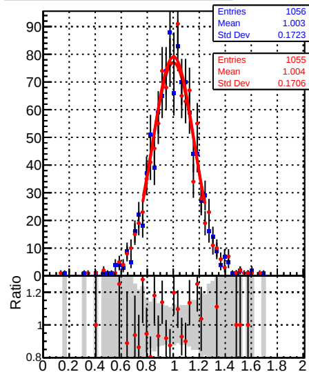
Jet response ( p_T/p_{T\text{gen}} ) in 84 \leq p_t < 114 , 2.5 \leq |\eta_{\text{jet}}| < 3.0
