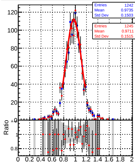
Jet response ( p_T/p_{T\text{gen}} ) in 84 \leq p_t < 114 , 2.1 \leq |\eta_{\text{jet}}| < 2.5
