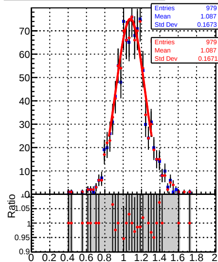
Jet response ( p_T/p_{T\text{gen}} ) in 84 \leq p_t < 114 , 3.0 \leq |\eta_{\text{jet}}| < 5.0
