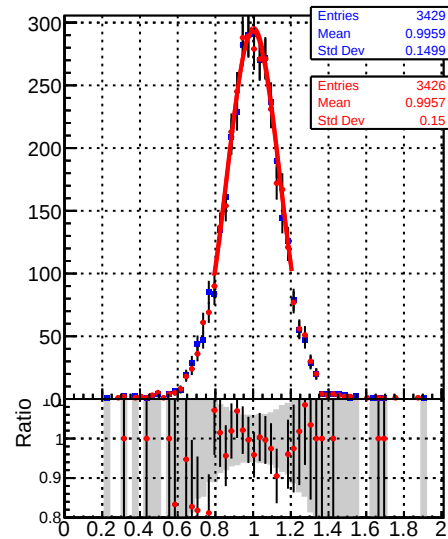
Jet response ( p_T/p_{T\text{gen}} ) in 84 \leq p_t < 114 , 1.3 \leq |\eta_{\text{jet}}| < 2.1
