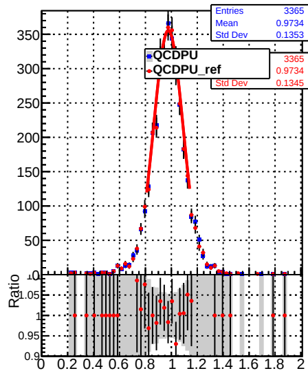
Jet response ( p_T/p_{T\text{gen}} ) in 84 \leq p_t < 114 , 0.5 \leq |\eta_{\text{jet}}| < 0.5
