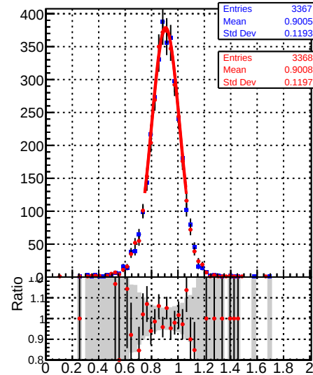
Raw Jet response (pT/pTgen) in 114 &lt;= pt &lt; 153, 1.3 &lt;= |eta| &lt; 2.1
