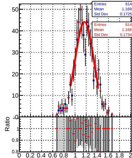
Raw Jet response (pT/pTgen) in 114 &lt;= pt &lt; 153, 3.0 &lt;= |eta| &lt; 5.0
