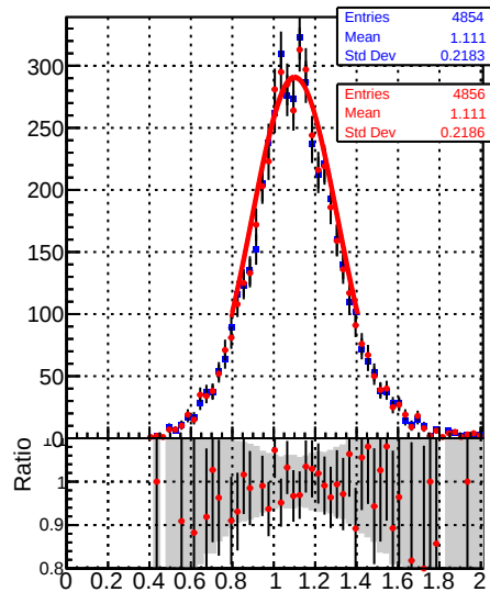
Raw Jet response (pT/pTgen) in 28 \leq p_t < 37, 0.5 \leq |\eta| < 2.1
