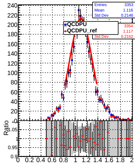
Raw Jet response (pT/pTgen) in 28 \leq p_t < 37, 0.0 \leq |\eta| < 2.5
