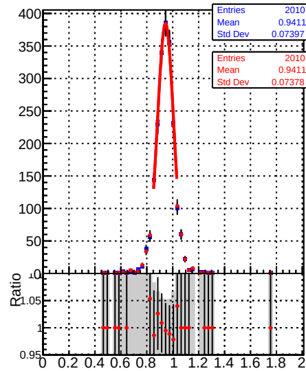
Raw Jet response (pT/pTgen) in 395 &lt;= pt &lt; 468, 0.5 &lt;= |eta| &lt; 1.3
