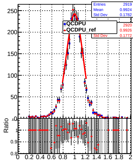
Jet response (pT/pTgen) in 49 \leq p_t < 64 , 0 \leq |\eta| < 0.5
