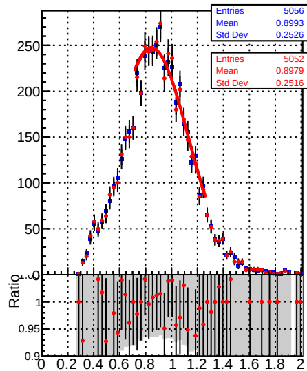
Raw Jet response (pT/pT gen ) in 21 <= pt < 28, 0.5 <= |eta| < 1.3
