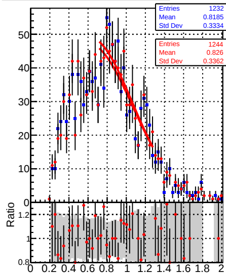
Raw Jet response (pT/pT gen ) in 21 <= pt < 28, 2.5 <= |eta| < 3.0
