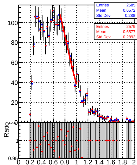
Raw Jet response (pT/pT gen ) in 21 <= pt < 28, 3.0 <= |eta| < 5.0
