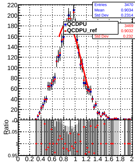
Raw Jet response (pT/pT gen ) in 21 <= pt < 28, 0.0 <= |eta| < 0.5
