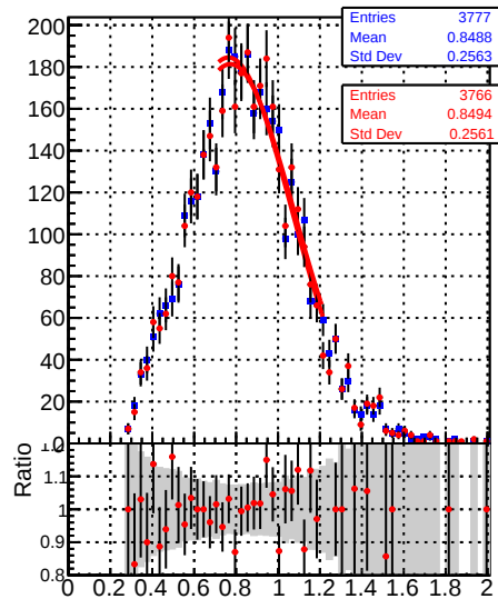
Raw Jet response (pT/pT gen ) in 21 <= pt < 28, 1.3 <= |eta| < 2.1
