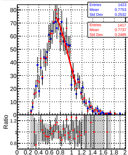
Raw Jet response (pT/pT gen ) in 21 <= pt < 28, 2.1 <= |eta| < 2.5
