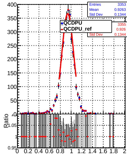
Raw Jet response (pT/pTgen) in 84 &lt;= pt &lt; 114, 0.0 &lt;= |eta| &lt; 0.5
