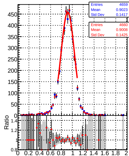
Raw Jet response (pT/pTgen) in 84 &lt;= pt &lt; 114, 0.5 &lt;= |eta| &lt; 1.3
