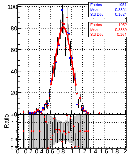
Raw Jet response (pT/pTgen) in 84 &lt;= pt &lt; 114, 2.5 &lt;= |eta| &lt; 3.0
