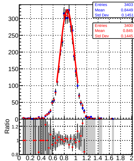
Raw Jet response (pT/pTgen) in 84 &lt;= pt &lt; 114, 1.3 &lt;= |eta| &lt; 2.1
