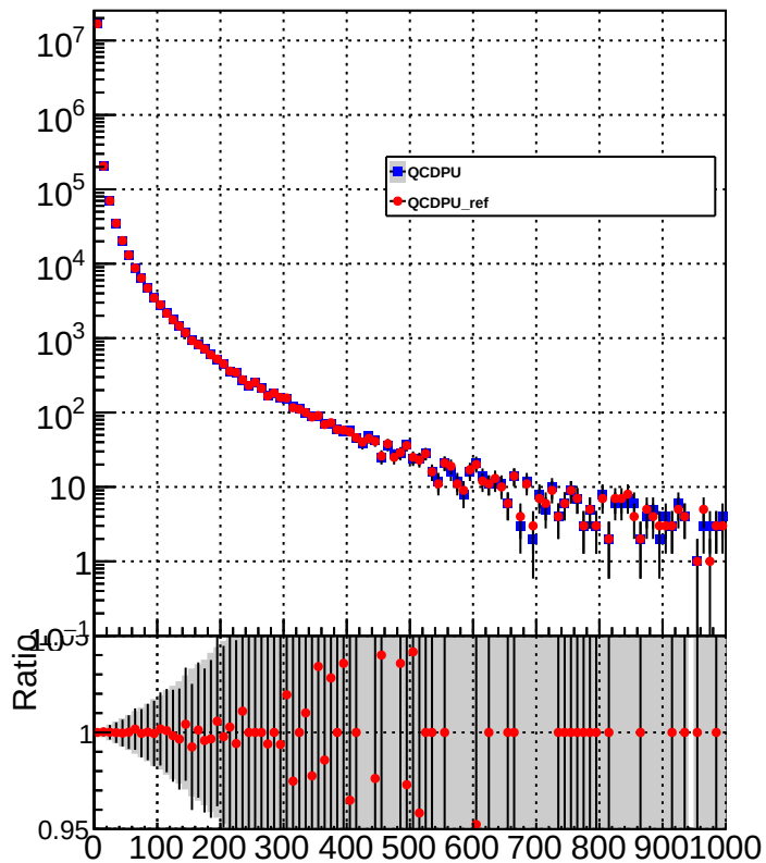
chargedHadronPtHigh
