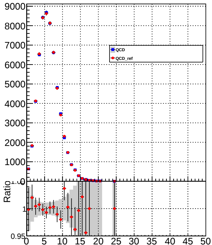
neutralHadronMultiplicity
