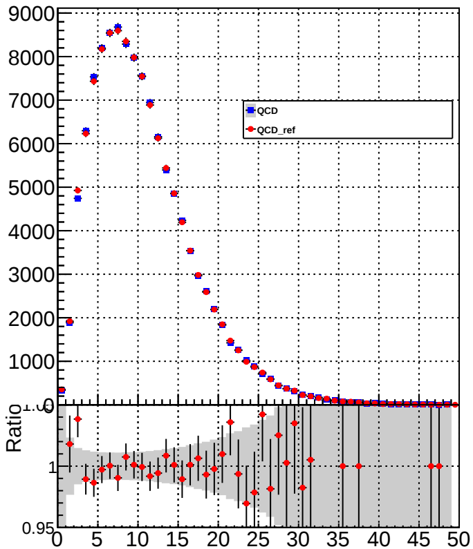
neutralMultiplicity
