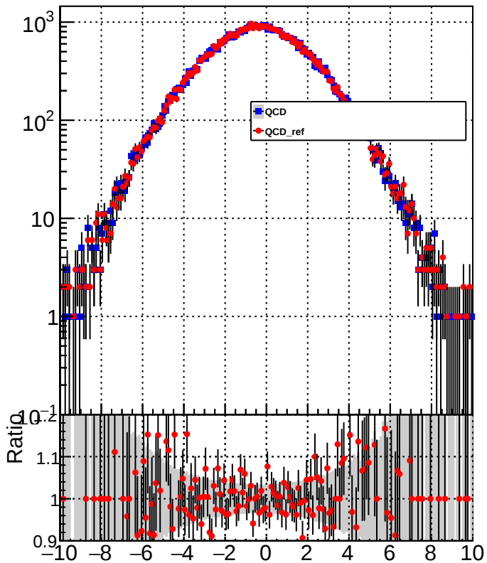
METUnc_UnclusteredEnUp
