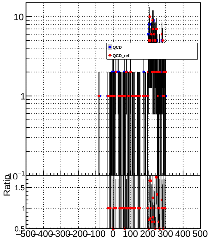
METResolution_GenMETTrue_MET200to300
