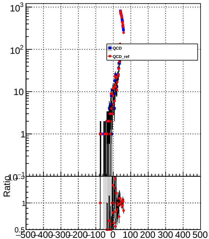
METResolution_GenMETTrue_MET40to60
