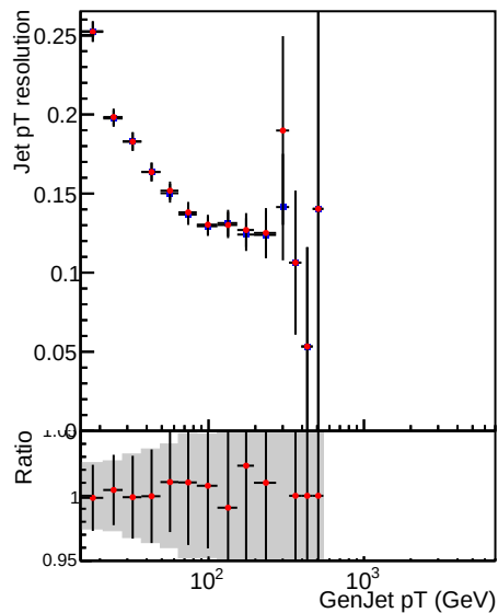
Jet pT resolution, 3.0 < |\eta| < 5.0
