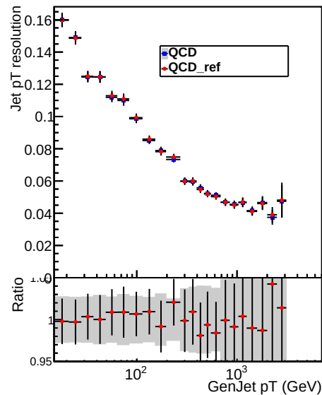
Jet pT resolution, 2.1 < |\eta| < 2.5
