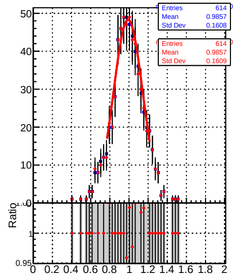
Raw Jet response (pT/pTgen) in 114 &lt;= pt &lt; 153, 3.0 &lt;= |eta| &lt; 5.0
