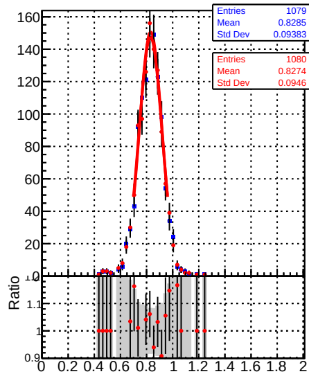
Raw Jet response (pT/pTgen) in 114 &lt;= pt &lt; 153, 2.1 &lt;= |eta| &lt; 2.5
