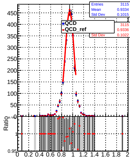
Raw Jet response (pT/pTgen) in 114 &lt;= pt &lt; 153, 0.0 &lt;= |eta| &lt; 0.5
