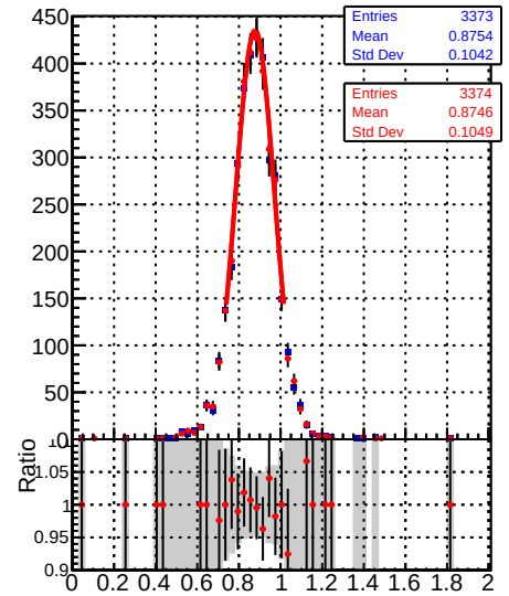
Raw Jet response (pT/pTgen) in 114 &lt;= pt &lt; 153, 1.3 &lt;= |eta| &lt; 2.1
