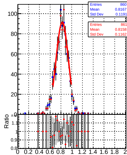
Raw Jet response (pT/pTgen) in 114 &lt;= pt &lt; 153, 2.5 &lt;= |eta| &lt; 3.0
