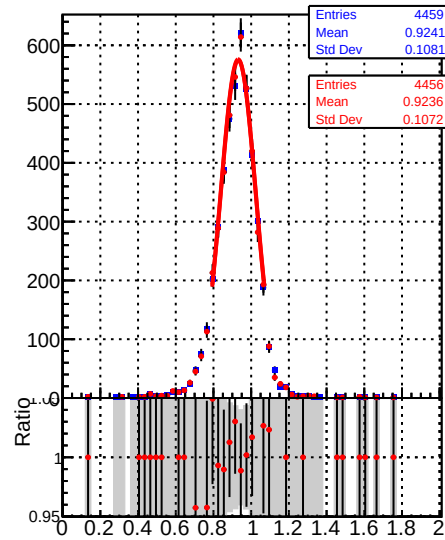
Raw Jet response (pT/pTgen) in 114 &lt;= pt &lt; 153, 0.5 &lt;= |eta| &lt; 1.3
