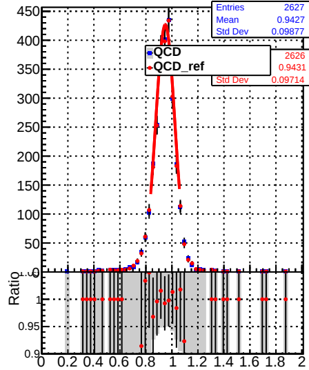
Raw Jet response (pT/pTgen) in 153 \leq p_t < 196, 0.0 \leq |\eta| < 0.5
