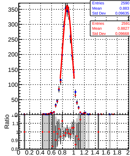
Raw Jet response (pT/pTgen) in 153 \leq p_t < 196, 1.3 \leq |\eta| < 2.1
