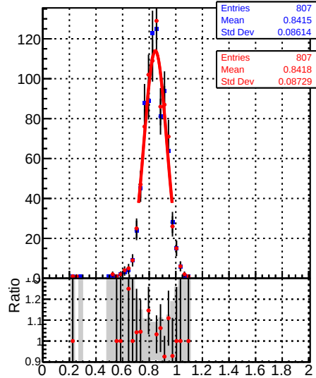
Raw Jet response (pT/pTgen) in 153 \leq p_t < 196, 2.1 \leq |\eta| < 2.5
