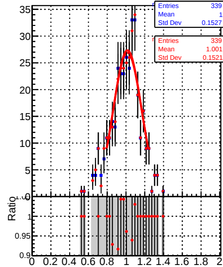
Raw Jet response (pT/pTgen) in 153 \leq p_t < 196, 3.0 \leq |\eta| < 5.0
