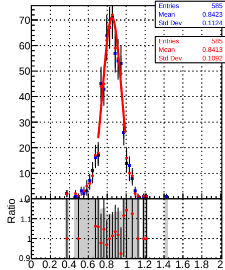
Raw Jet response (pT/pTgen) in 153 \leq p_t < 196, 2.5 \leq |\eta| < 3.0
