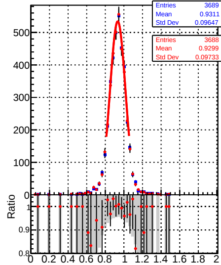
Raw Jet response (pT/pTgen) in 153 \leq p_t < 196, 0.5 \leq |\eta| < 1.3
