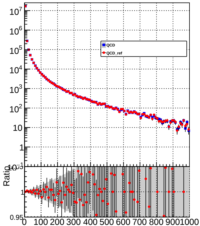
AllCandidatePtHigh
