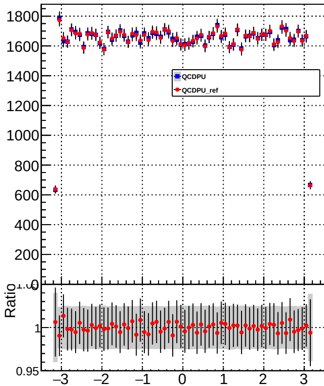
CorrJetPhi Pt>40
