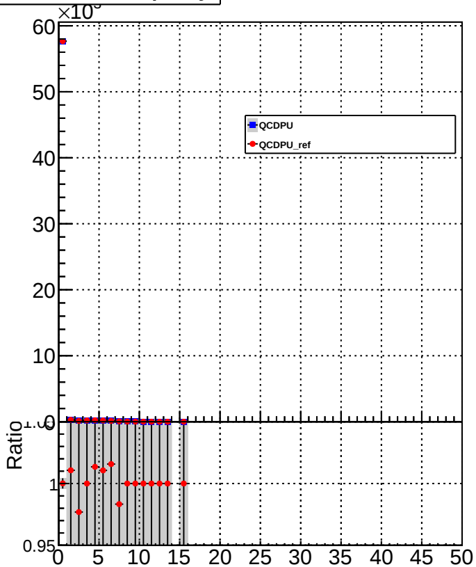
HFHadronMultiplicity
