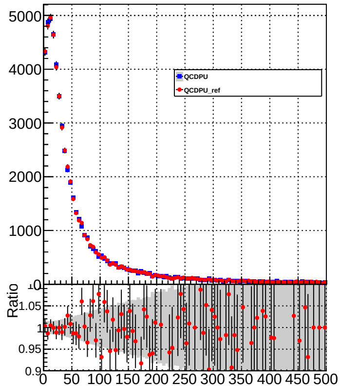
neutralHadronEnergy
