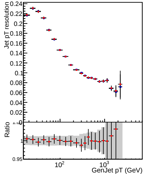
Raw Jet pT resolution using RMS, 3.0 < |\eta| < 5.0
