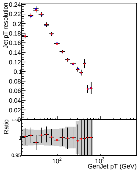
Raw Jet pT resolution using RMS, 2.5 < |\eta| < 3.0
