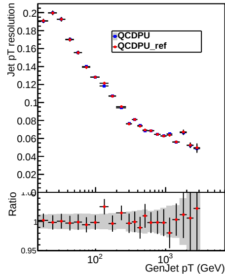
Raw Jet pT resolution using RMS, 2.1 < |\eta| < 2.5
