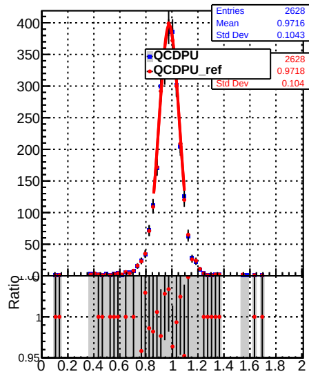
Raw Jet response (pT/pTgen) in 153 \leq p_t < 196 , 0.0 \leq |\eta| < 2.5
