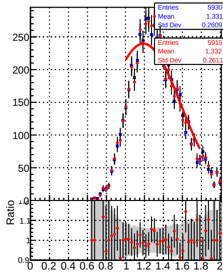
Raw Jet response (pT/pTgen) in 15 \leq p_t < 21, 0.5 \leq |\eta| < 1.3
