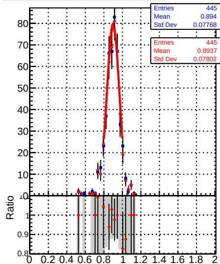
Raw Jet response (pT/pTgen) in 272 &lt;= pt &lt; 330, 2.1 &lt;= |eta| &lt; 2.5
