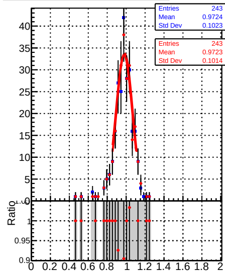
Raw Jet response (pT/pTgen) in 272 &lt;= pt &lt; 330, 2.5 &lt;= |eta| &lt; 3.0
