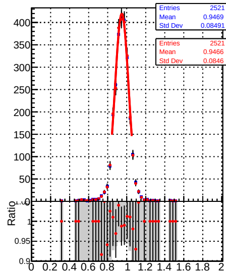
Raw Jet response (pT/pTgen) in 272 &lt;= pt &lt; 330, 0.5 &lt;= |eta| &lt; 1.3
