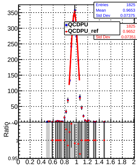
Raw Jet response (pT/pTgen) in 272 &lt;= pt &lt; 330, 0.0 &lt;= |eta| &lt; 0.5
