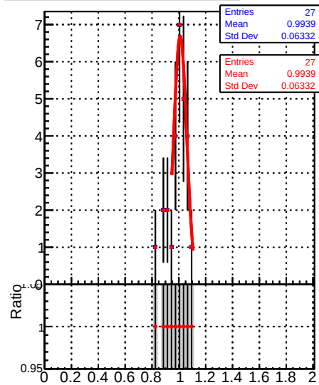
Raw Jet response (pT/pTgen) in 468 &lt;= pt &lt; 548, 2.5 &lt;= |eta| &lt; 3.0
