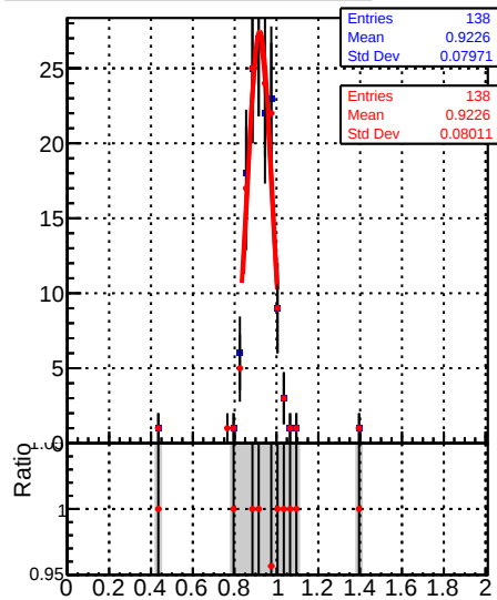
Raw Jet response (pT/pTgen) in 468 &lt;= pt &lt; 548, 2.1 &lt;= |eta| &lt; 2.5
