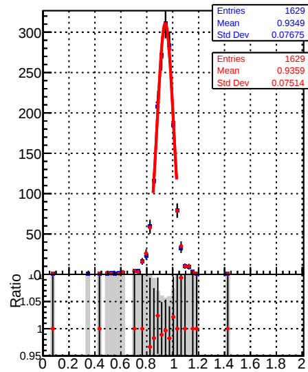
Raw Jet response (pT/pTgen) in 468 &lt;= pt &lt; 548, 0.5 &lt;= |eta| &lt; 1.3
