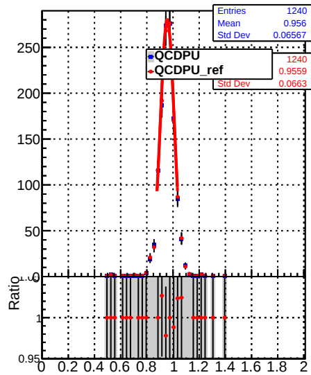
Raw Jet response (pT/pTgen) in 468 &lt;= pt &lt; 548, 0.0 &lt;= |eta| &lt; 0.5
