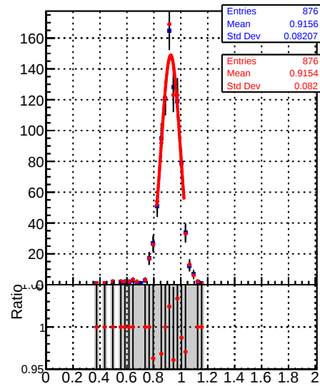
Raw Jet response (pT/pTgen) in 468 &lt;= pt &lt; 548, 1.3 &lt;= |eta| &lt; 2.1
