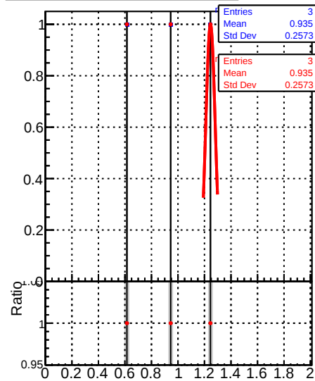
Raw Jet response (pT/pTgen) in 468 &lt;= pt &lt; 548, 3.0 &lt;= |eta| &lt; 5.0
