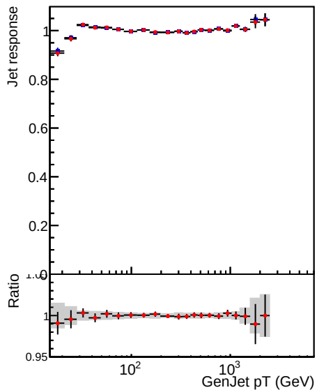
Jet pT response, 3.0 < |\eta| < 5.0
