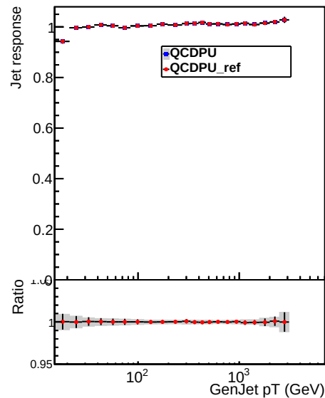
Jet pT response, 2.1 < |\eta| < 2.5
