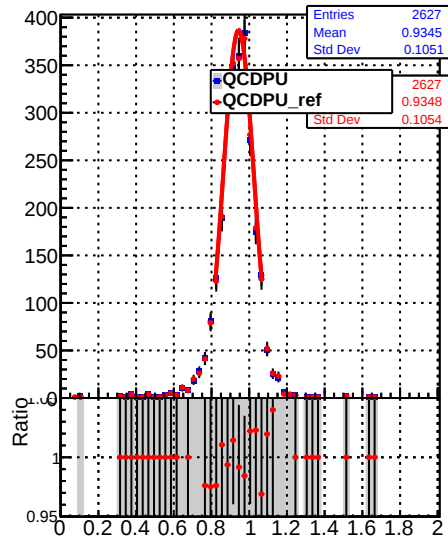
Raw Jet response ( pT/pT_{\text{gen}} ) in 153 \leq p_t \leq 196 , 0.0 \leq |\eta| \leq 2.5
