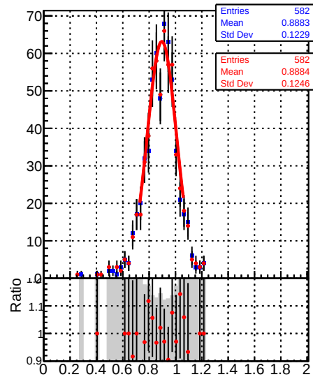
Raw Jet response ( pT/pT_{\text{gen}} ) in 153 \leq p_t \leq 196 , 2.5 \leq |\eta| \leq 3.0
