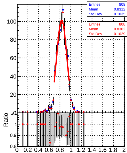
Raw Jet response ( pT/pT_{\text{gen}} ) in 153 \leq p_t \leq 196 , 2.1 \leq |\eta| \leq 2.5
