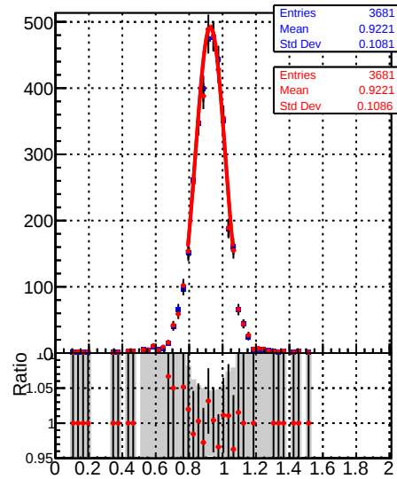
Raw Jet response ( pT/pT_{\text{gen}} ) in 153 \leq p_t \leq 196 , 0.5 \leq |\eta| \leq 1.3
