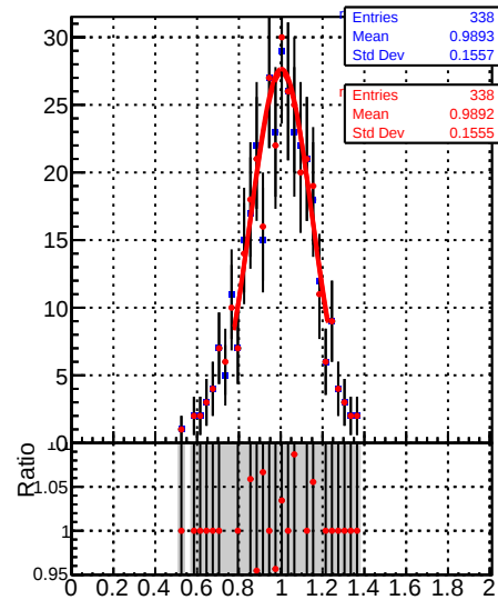
Raw Jet response ( pT/pT_{\text{gen}} ) in 153 \leq p_t \leq 196 , 3.0 \leq |\eta| \leq 5.0
