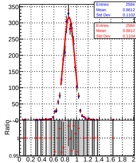
Raw Jet response ( pT/pT_{\text{gen}} ) in 153 \leq p_t \leq 196 , 1.3 \leq |\eta| \leq 2.1
