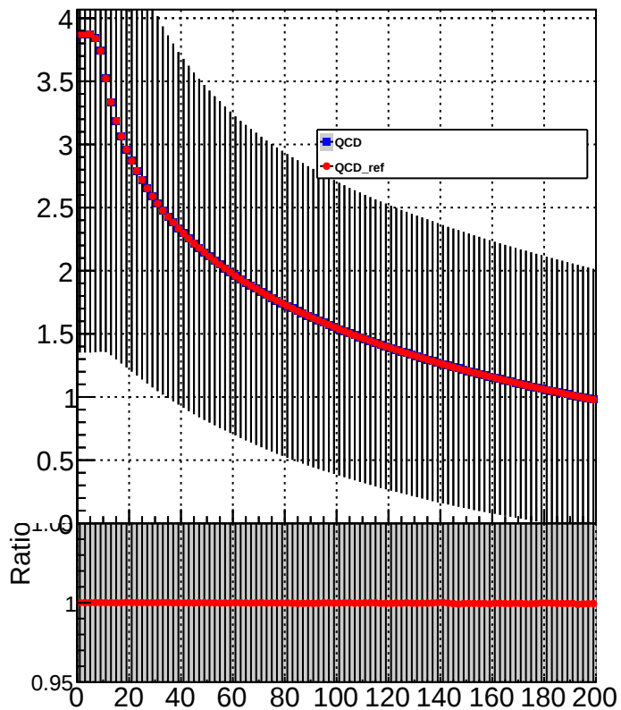
Number of jets above Pt threshold
