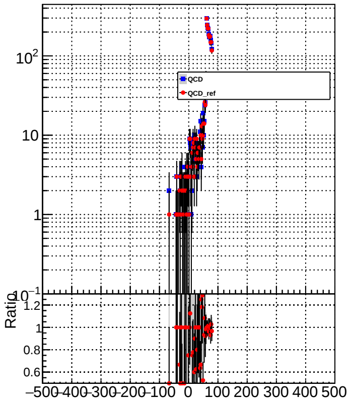
METResolution_GenMETTrue_MET60to80
