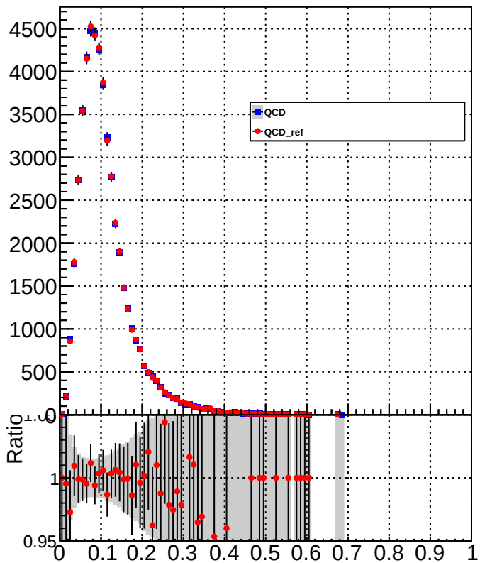
neutralHadronEtFraction
