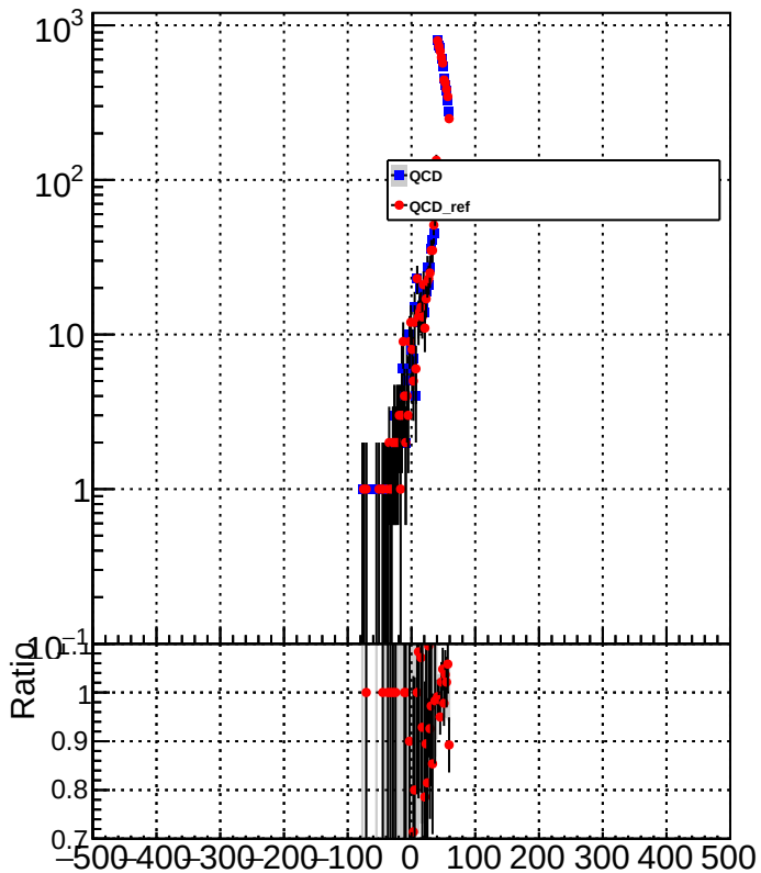
METResolution_GenMETTrue_MET40to60
