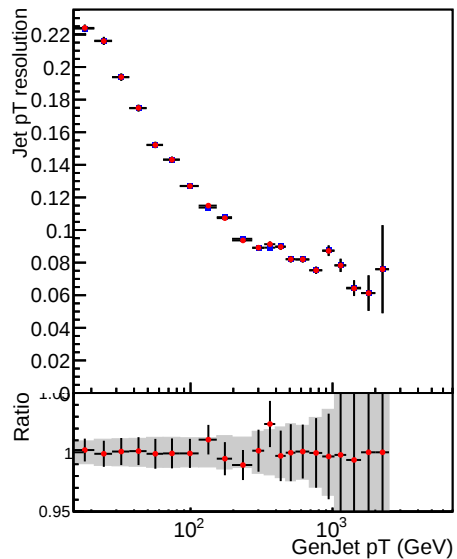
Jet pT resolution using RMS, 3.0 < |\eta| < 5.0
