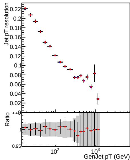
Jet pT resolution using RMS, 2.1 < |\eta| < 2.5
