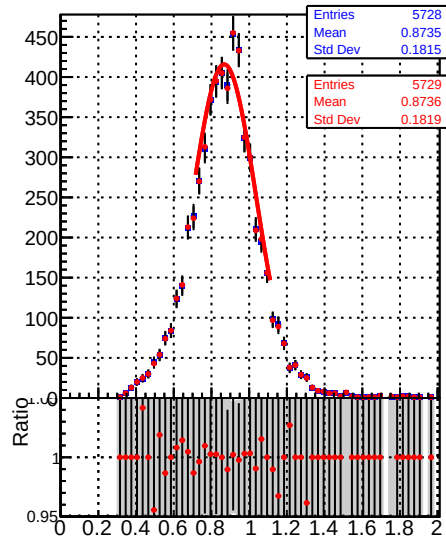
Raw Jet response (pT/pTgen) in 21 \leq p_t < 28, 0.5 \leq |\eta| < 2.1
