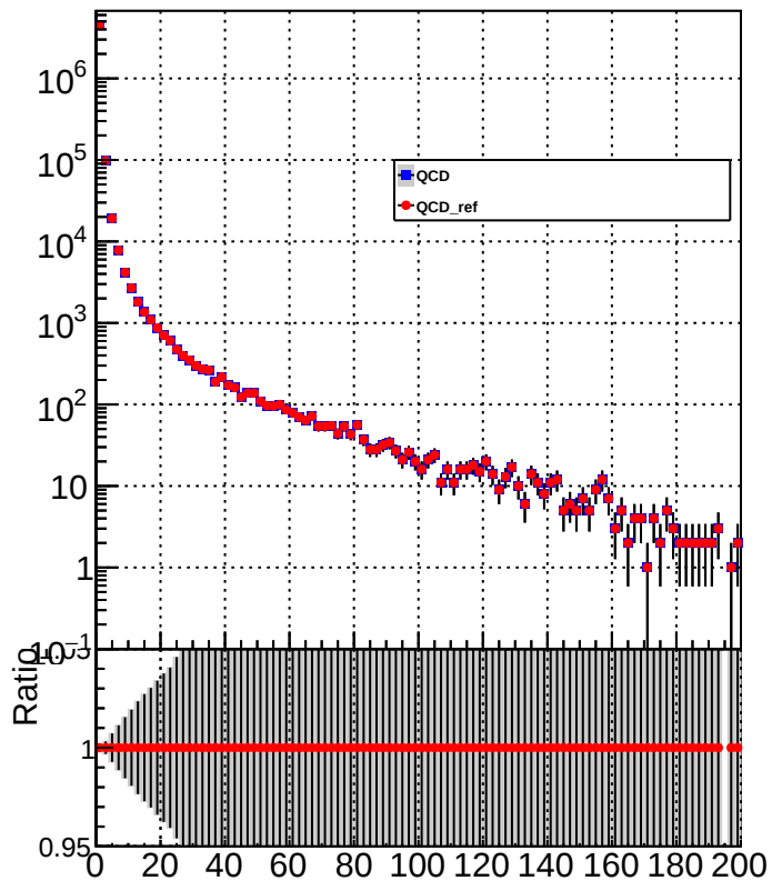
HF_hadronPtMid
