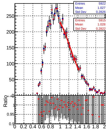
Jet response ( p_T/p_{T\text{gen}} ) in 15 \leq p_T < 21 , 0.5 \leq |\eta| < 1.3
