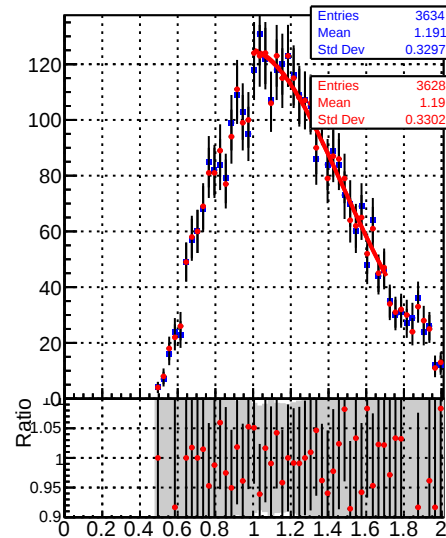
Jet response ( p_T/p_{T\text{gen}} ) in 15 \leq p_T < 21 , 3.0 \leq |\eta| < 5.0
