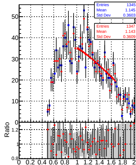
Jet response ( p_T/p_{T\text{gen}} ) in 15 \leq p_T < 21 , 2.5 \leq |\eta| < 3.0
