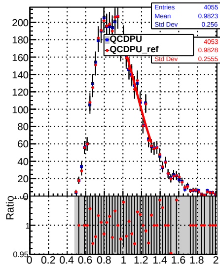
Jet response ( p_T/p_{T\text{gen}} ) in 15 \leq p_T < 21 , 0.0 \leq |\eta| < 0.5
