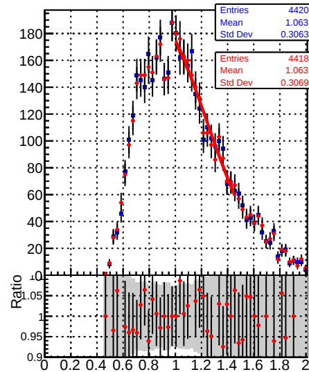
Jet response ( p_T/p_{T\text{gen}} ) in 15 \leq p_T < 21 , 1.3 \leq |\eta| < 2.1
