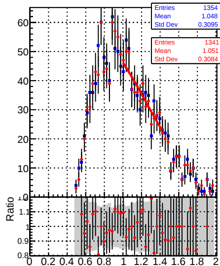
Jet response ( p_T/p_{T\text{gen}} ) in 15 \leq p_T < 21 , 2.1 \leq |\eta| < 2.5
