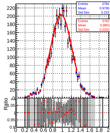
Jet response (pT/pTgen) in 37 \leq p_t < 49, 1.0 \leq |\eta| < 1.5
