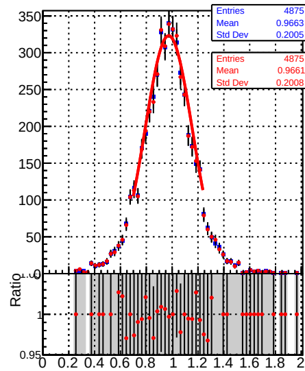
Jet response (pT/pTgen) in 37 \leq p_t < 49, 0.5 \leq |\eta| < 1.0
