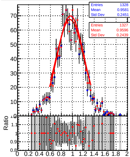
Jet response (pT/pTgen) in 37 \leq p_t < 49, 2.0 \leq |\eta| < 2.5
